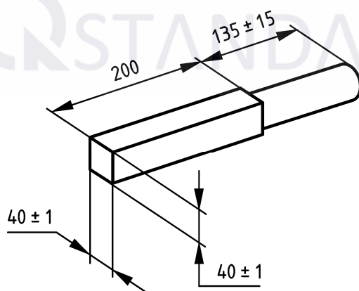
Figure 3 — Tamping bar
